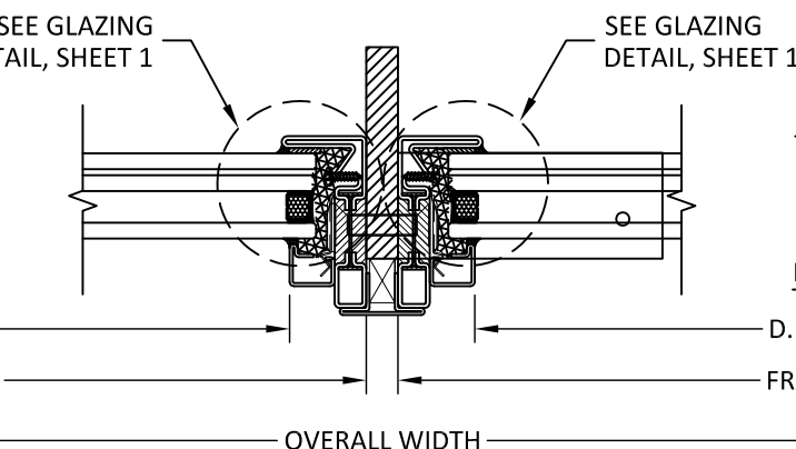
E 6 HORIZONTAL SECTION MULLION - OUTSIDE GLAZED
