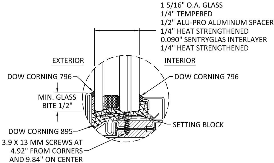
GLAZING DETAIL 1 INSIDE GLAZED
