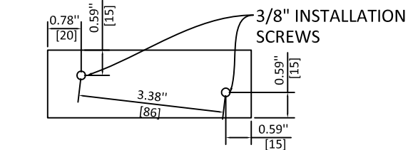
MULL CLIP ANCHOR LAYOUT CONCRETE SUBSTRATE
