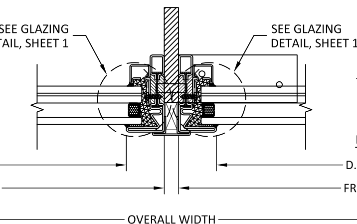
B 6 HORIZONTAL SECTION MULLION - INSIDE GLAZED
