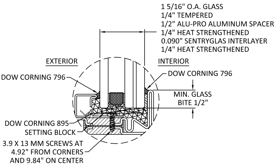
GLAZING DETAIL 2 OUTSIDE GLAZED
