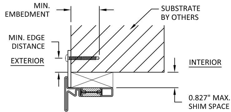
C 7 ANCHOR DETAIL NAIL FIN
