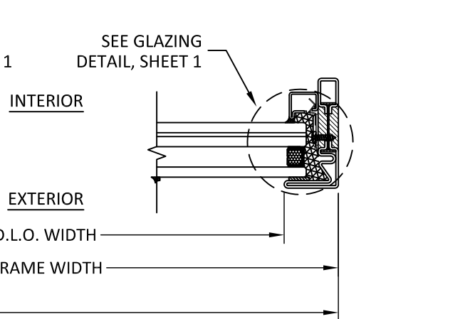
C 6 HORIZONTAL SECTION JAMB - INSIDE GLAZED
