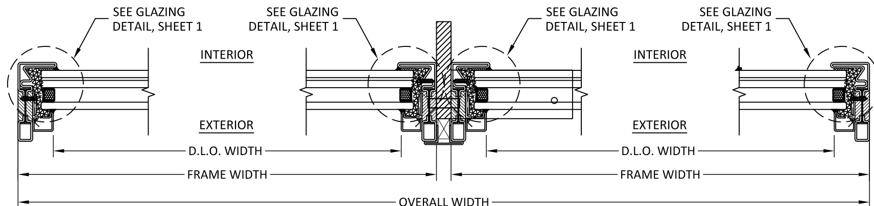
D 6 HORIZONTAL SECTION JAMB - OUTSIDE GLAZED
