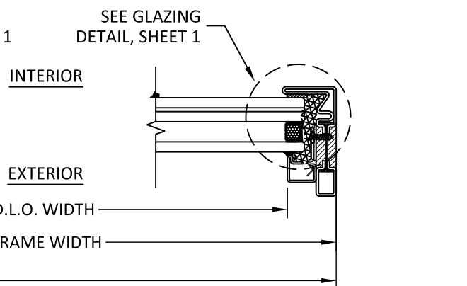
F 6 HORIZONTAL SECTION JAMB - OUTSIDE GLAZED
