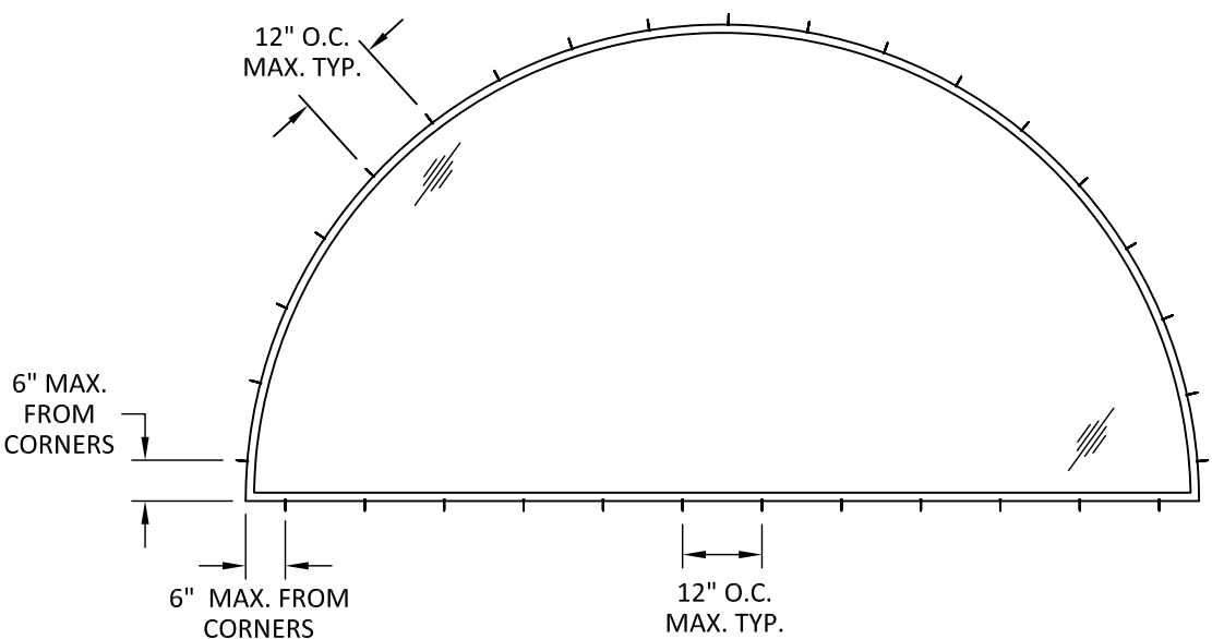
ANCHOR LAYOUT
