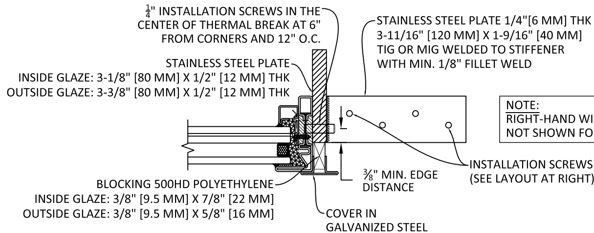
D 7 MULLION ANCHOR DETAIL MULL CLIP
