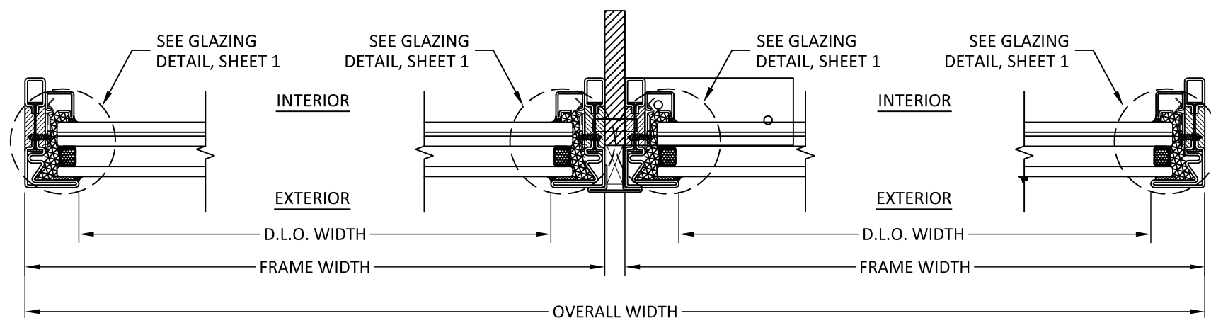
A 6 HORIZONTAL SECTION JAMB - INSIDE GLAZED
